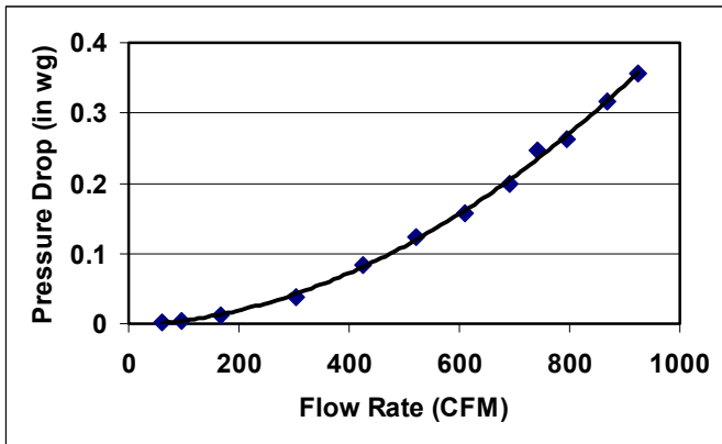
Figure 6. Characteristics of perforated tile
