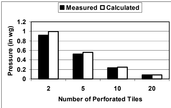
Figure 13. Average plenum pressure, seams are sealed
