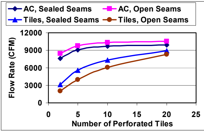
Figure 8. A/C unit and perforated tiles flow rates for two cases of sealed seams and open seams
