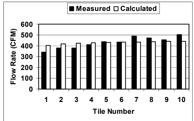
Figure 16. Airflow through one row of perforated tiles, seams are sealed
