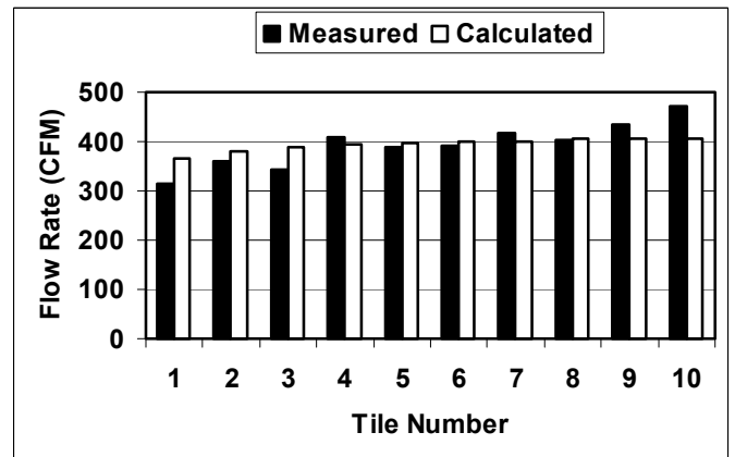
Figure 17. Airflow through one row of perforated tiles, seams are open
