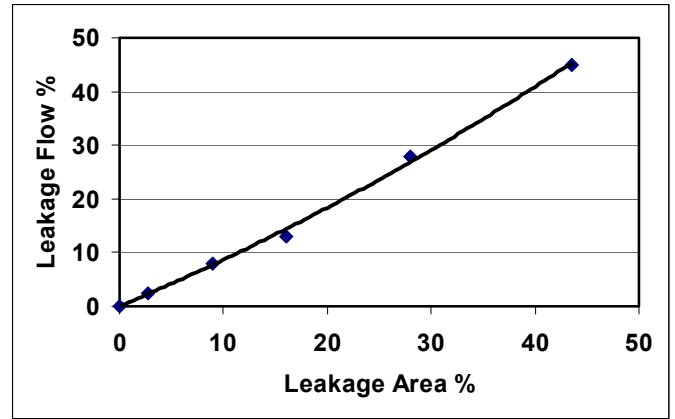
Figure 11. Non-dimensional leakage flow as a function of non-dimensional leakage area.
