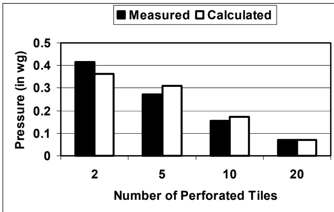
Figure 14. Average plenum pressure, seams are open
