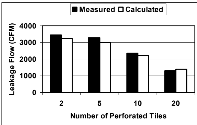
Figure 15. Distributed leakage flow
