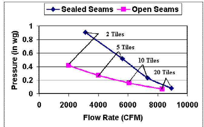
Figure 7. Plenum pressure vs. total flow rate through perforated tiles for different number of perforated tiles
