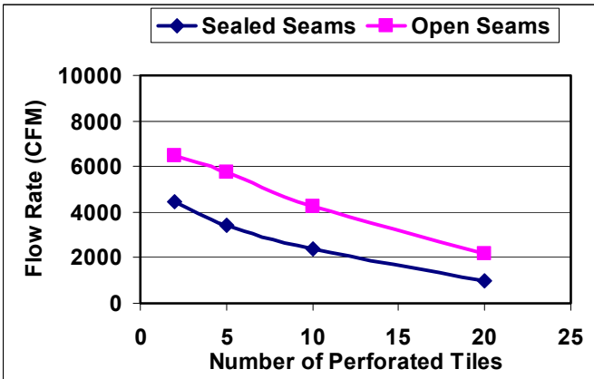
Figure 9. Total leakage flow rate for two cases of sealed seams and open seams
