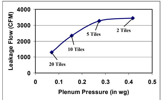
Figure 10. Airflow leakage through seams between tiles
